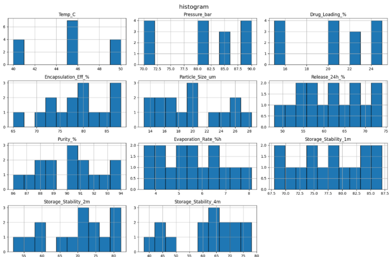
Figure 1. Histograms of Experimental Variables
