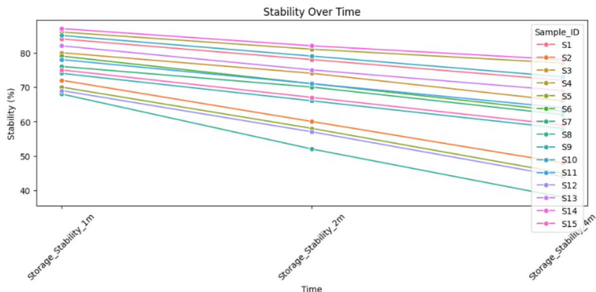
Figure 4. Interpretation of the Stability Over Time Chart
